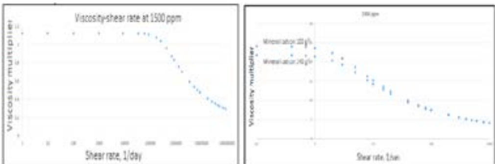
Fig. 3 – Viscosity – shear rate at 1500 ppm, 2000 ppm
